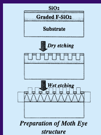
Moth Eye structure F-SiO 2 glass thin film on Si
