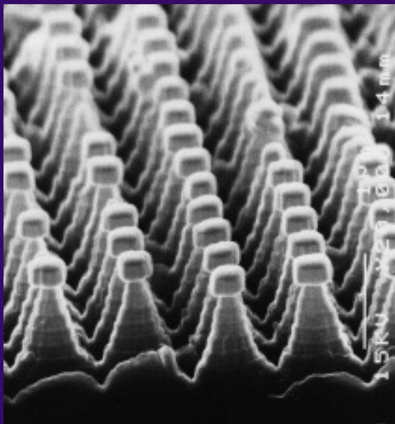
Moth Eye structure F-SiO 2 glass thin film on Si
