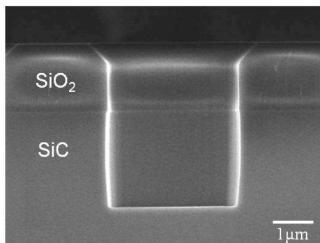
Figure 5. SiC trench etching result from optimized SiC trench etching process.
