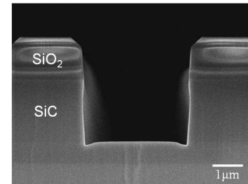
(b) Bias = 500W, electrode gap = 90 mm SiC etching rate = 412 nm/min, etch selectivity (SiC/SiO 2 ) = 4.6
