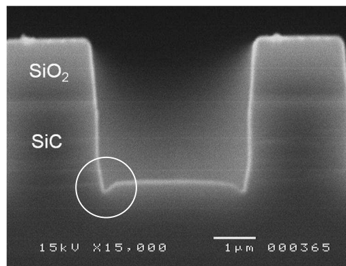
Figure 1. A 3.5 \mu\text{m} wide SiC trench etching result from an early SiC trench etching experiment in another ICP etching system, showing micro-trenches (white circle).
