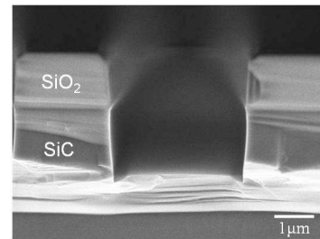
(a) Bias = 300W, electrode gap = 90 mm SiC etching rate = 330 nm/min, etch selectivity (SiC/SiO 2 ) = 4.6
