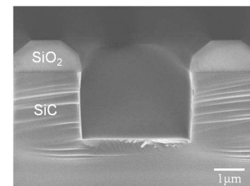
(c) Bias = 500W, electrode gap = 170 mm SiC etching rate = 438 nm/min, etch selectivity (SiC/SiO 2 ) = 2.8
