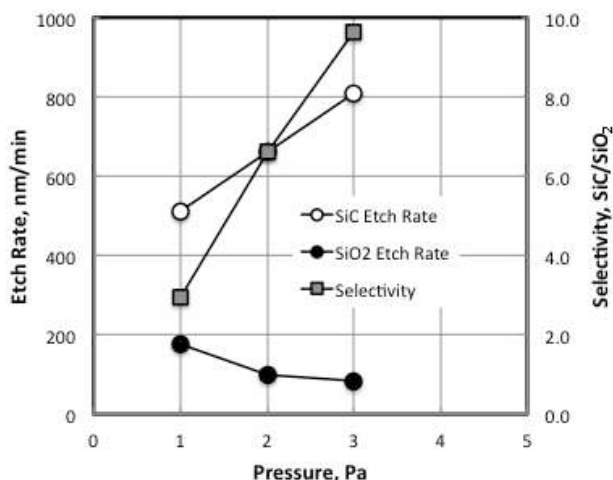
Figure 4. SiC etch rate and SiC/SiO 2 selectivity versus the process pressure
